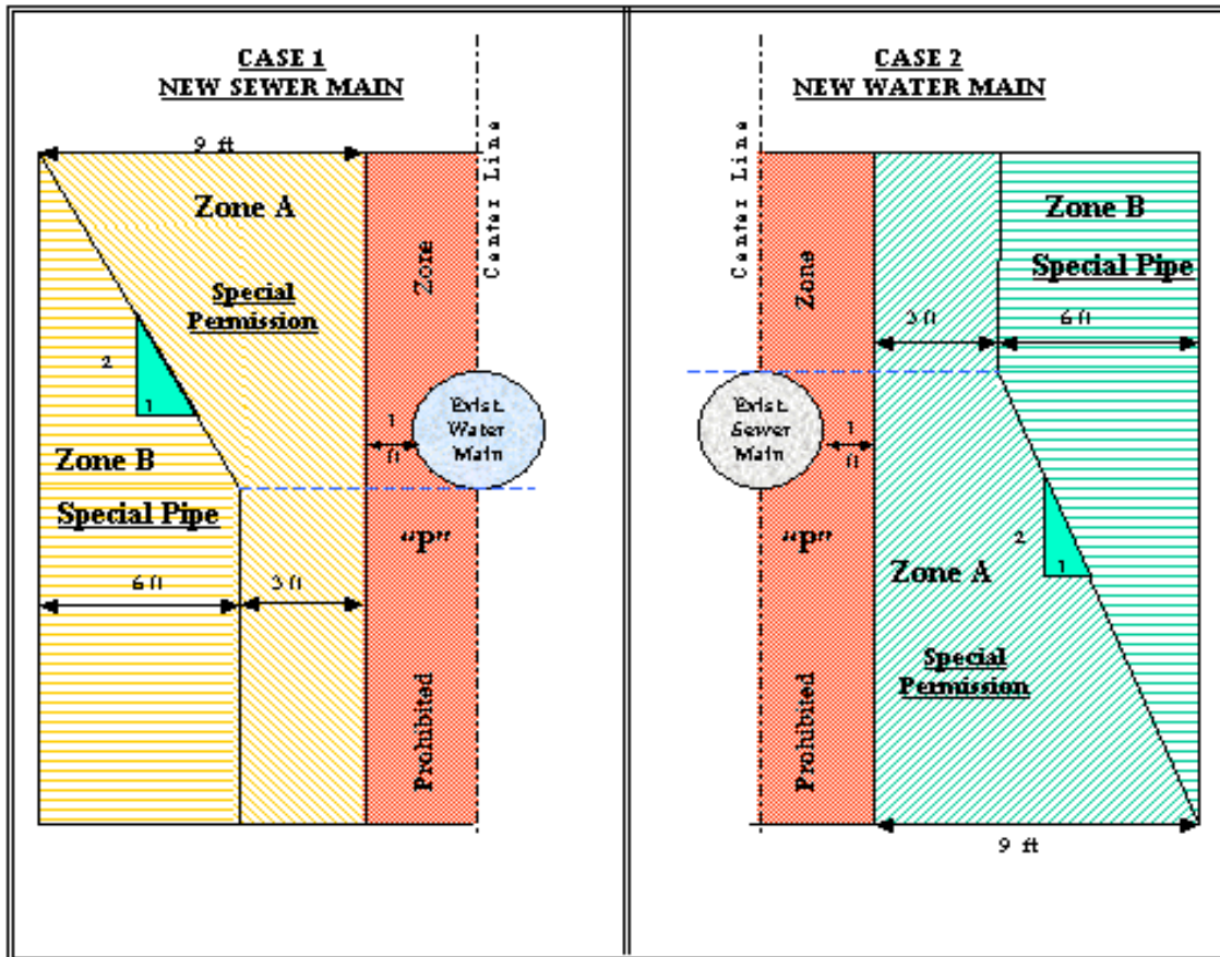
FIGURE 1 PARALLEL CONSTRUCTION
